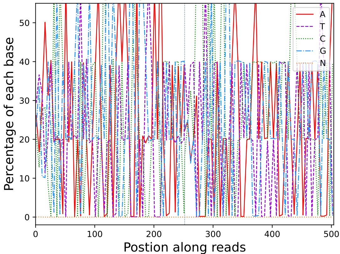
Base percentage along reads (R10525)
